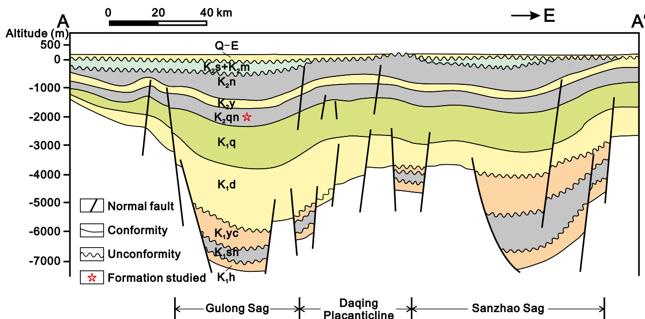
Figure 2. Transverse section across the middle segment of the Gulong sag, Daqing placanticline, and Sanzhao sag. E = Paleogene; K 1 d = Lower Cretaceous Denglouku Formation; K 1 h = Lower Cretaceous Huoshiling Formation; K 1 q = Lower Cretaceous Quantou Formation; K 1 sh = Lower Cretaceous Shahezi Formation; K 1 yc = Lower Cretaceous Yingcheng Formation; K 2 m = Upper Cretaceous Mingshui Formation; K 2 n = Upper Cretaceous Nenjiang Formation; K 2 qn = Upper Cretaceous Qingshankou Formation; K 2 s = Upper Cretaceous Sifangtai Formation; K 2 y = Upper Cretaceous Yaojia Formation; Q = Quaternary.
