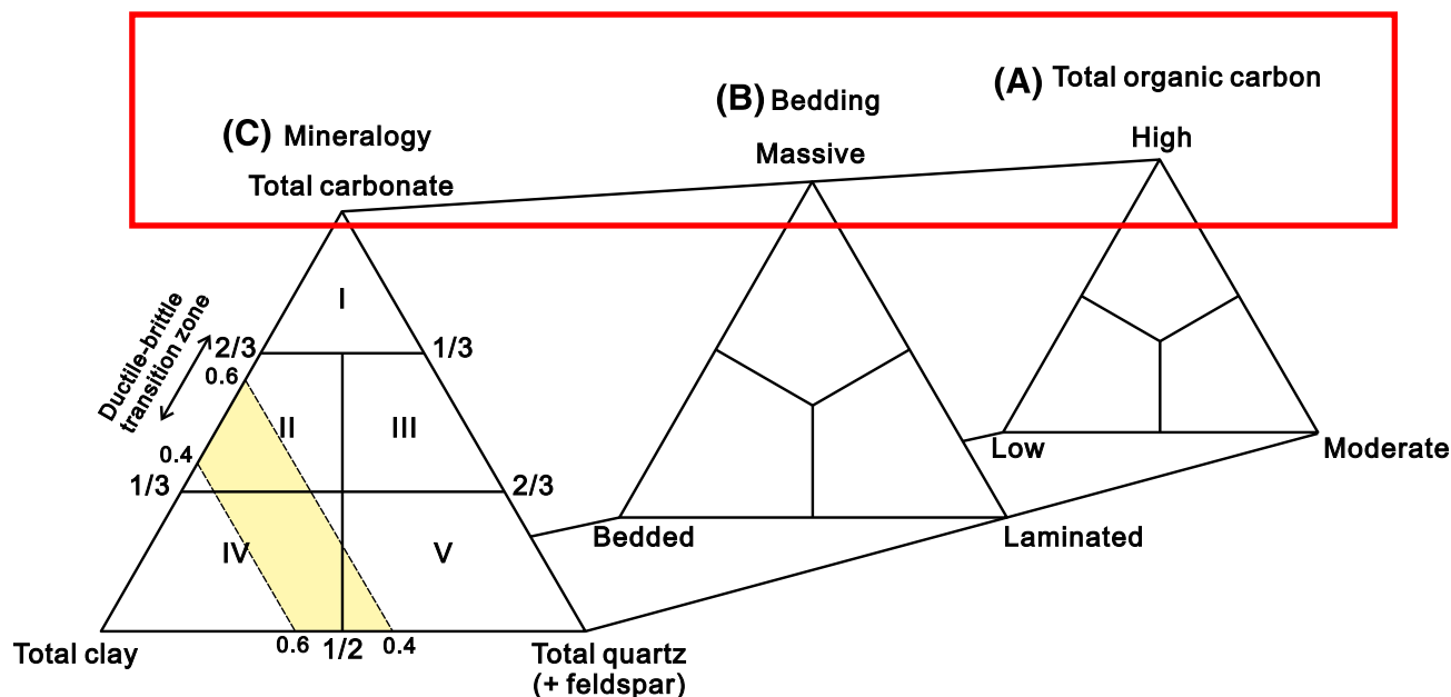
Figure 5. Classification of organic mudstones lithofacies using content of total organic carbon (rich, more than 2 wt. %; moderate, 1–2 wt. %; low, less than 1 wt. % [according to Allix et al., 2010; Anderson, 2014]) (A), bedding types (B), and mineral composition (C). I = calcareous mudstone; II = argillaceous marlstone; III = siliceous marlstone; IV = argillaceous mudstone (shale); V = siliceous mudstone.
