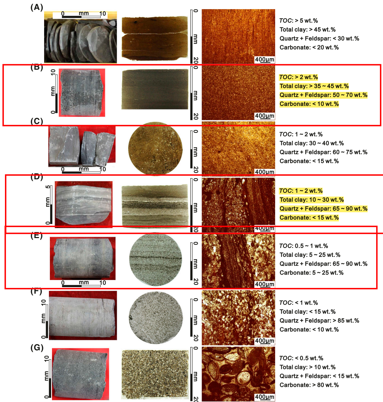
Figure 9. Lithofacies within the Qingshankou shale. Core image, thin section image, and transmitted light image show example of each individual facies. (A) High-total organic carbon (TOC) laminated argillaceous mudstone. (B) High-TOC massive siliceous mudstone. (C) Moderate-TOC massive siliceous mudstone. (D) Moderate-TOC laminated siliceous mudstone. (E) Low-TOC laminated siliceous mudstone. (F) Low-TOC bedded siliceous siltstone. (G) Low-TOC bedded calcareous mudstone. Each lithofacies description includes a range of TOC, total clay, quartz + feldspar, and carbonate.
