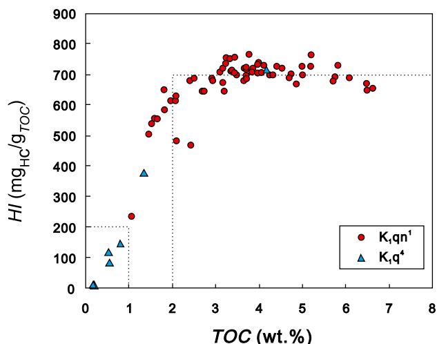
Figure 4. The total organic carbon ( TOC ) versus the hydrogen index ( HI ) of the immature Qingshankou Formation shales in one borehole (data from F. Wang et al., 2016). HC = hydrocarbon; K 1 qn 1 = the first member of the Qingshankou Formation; K 1 q 4 = the fourth member of Quantou Formation.
