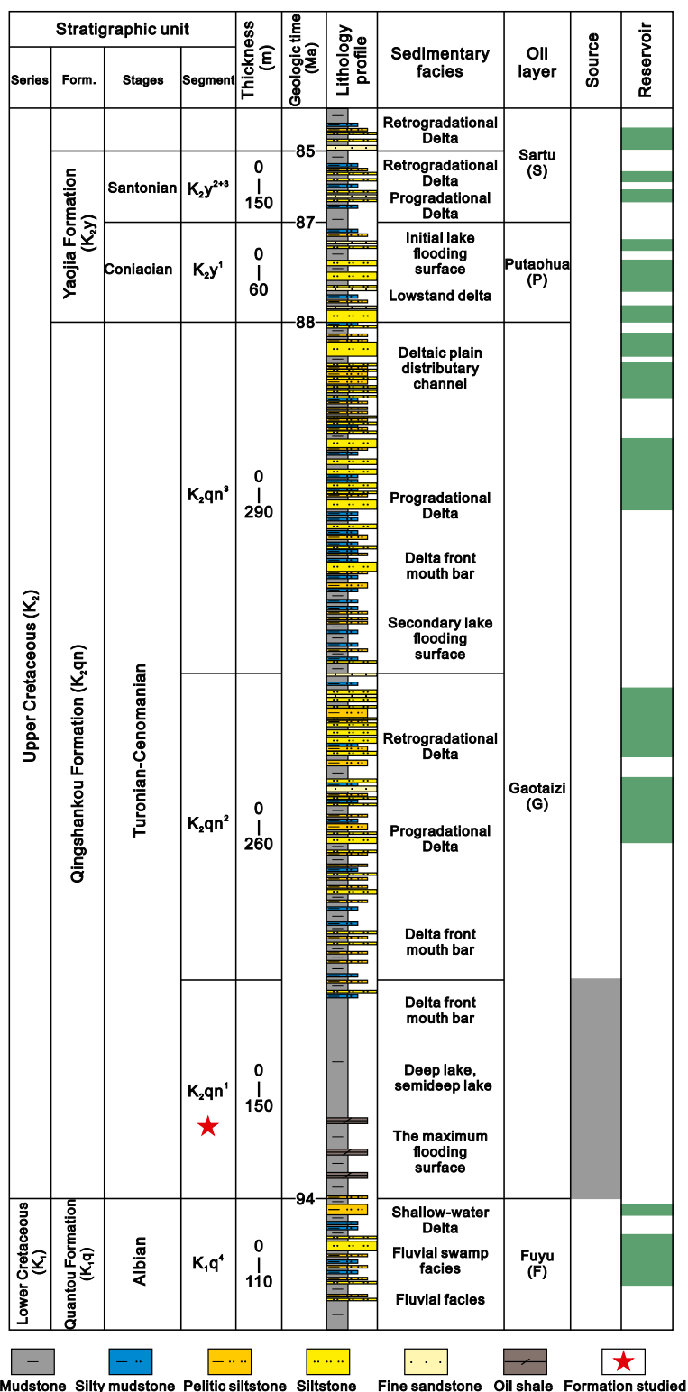
Figure 3. General lithologic stratigraphy of the Qingshankou Formation (Form.) in northern Songliao Basin. Gray and green in the column show the source and reservoir successions, respectively. K 1 q 4 = the fourth member of Quantou Formation; K 2 qn 1 = the first member of the Qingshankou Formation; K 2 qn 2 = the second member of the Qingshankou Formation; K 2 qn 3 = the third member of the Qingshankou Formation; K 2 y 1 = the first member of Yaojia Formation; K 2 y 2+3 = the second and third members of Yaojia Formation.
