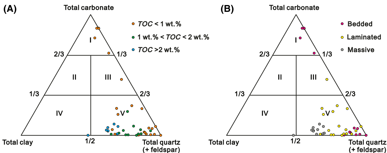
Figure 8. Ternary diagram showing mineral composition and total organic carbon (TOC) (A), and mineral composition and rock fabric (B) of the Qingshankou Formation shale in the northern Songliao Basin. I = calcareous mudstone; II = argillaceous marlstone; III = siliceous marlstone; IV = argillaceous mudstone (shale); V = siliceous mudstone.
