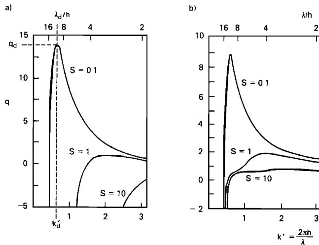
Fig. 3. Growth rate spectra for (a) viscous flexure and (b) hydrodynamic flow models for a range of S values. The dominant wave number k_d' and wavelength \lambda_d/h correspond to the maximum growth rate q_d for a given value of S . For S = 0.1 the dominant wavelengths are in good agreement. At larger S the dominant wavelengths deviate, indicating the breakdown of the thin plate approximations in the flexural buckling theory. Values of \alpha = 0.1 and n = 1 for the layer and substrate were assumed for both models. For the hydrodynamic flow model R = 1 .
